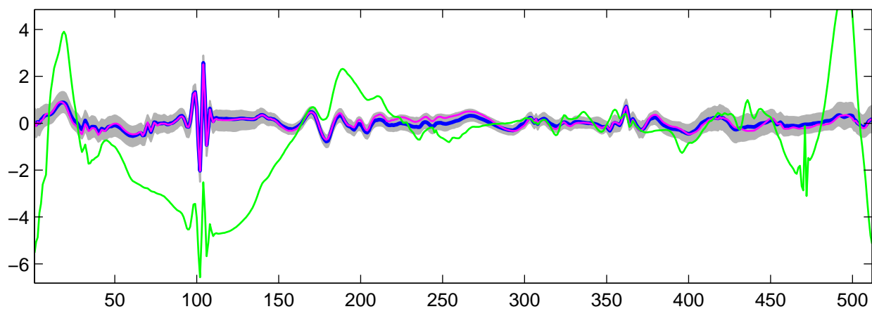
Estimated U_6(t) using R-WFMM: t_1 data, run 7
