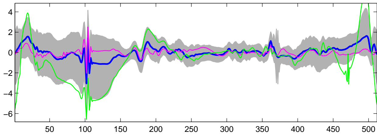
Estimated U_6(t) using G-WFMM: t_1 data, run 7
