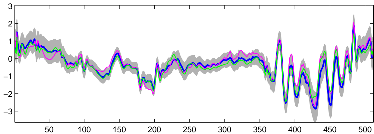
Estimated U_6(t) using R-WFMM: t_3 data, run 7
