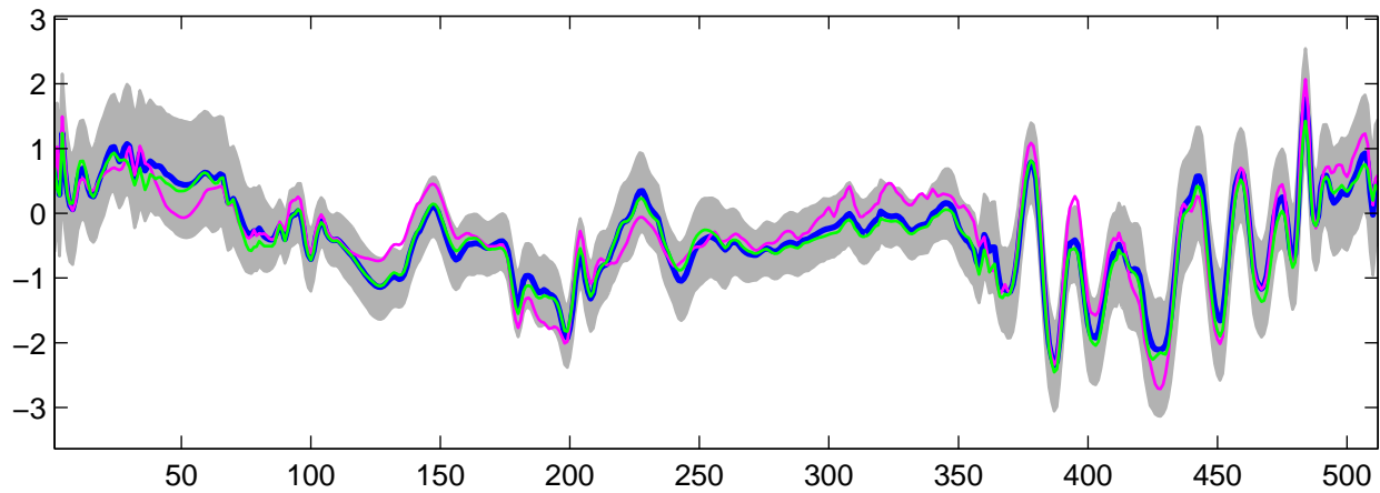
Estimated U_6(t) using G-WFMM: t_3 data, run 7
