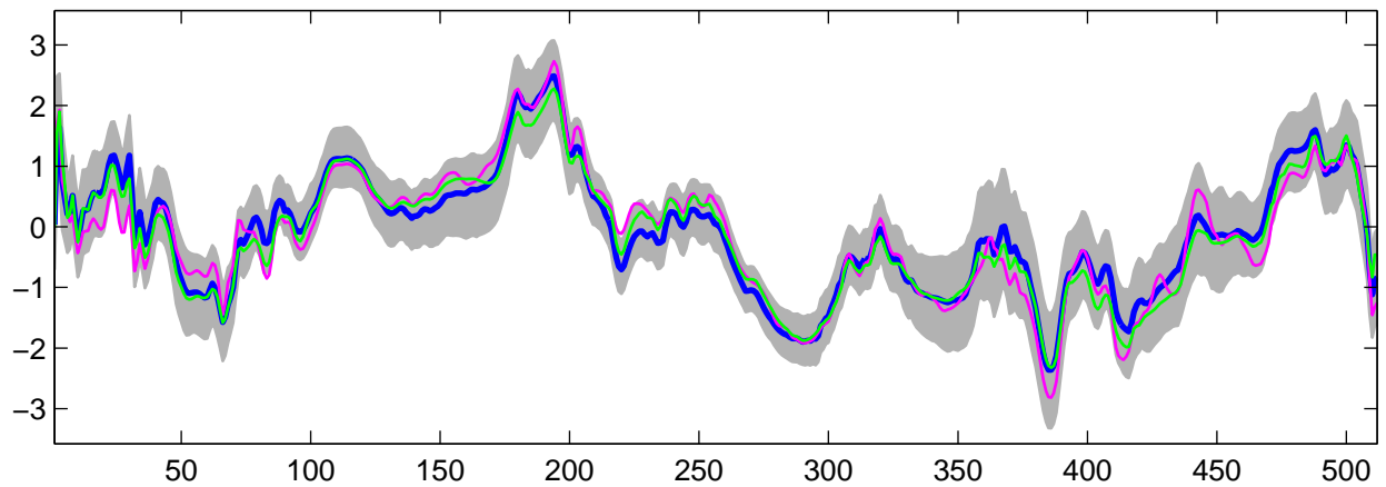
Estimated U_7(t) using R-WFMM: Normal data, run 7
