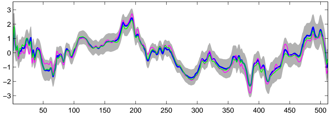
Estimated U_7(t) using G-WFMM: Normal data, run 7
