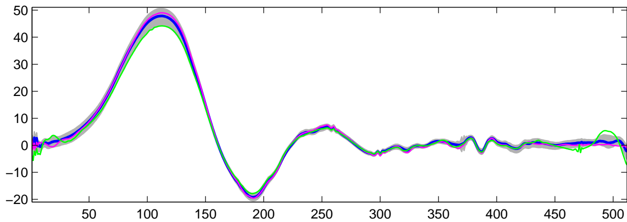
Estimated U_7(t) using G-WFMM: t_1 data, run 7
