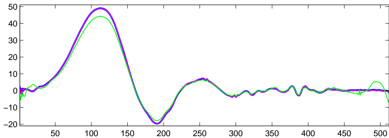
Estimated U_7(t) using R-WFMM: t_1 data, run 7
