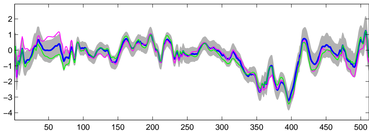
Estimated U_g(t) using R-WFMM: DE data, run 7
