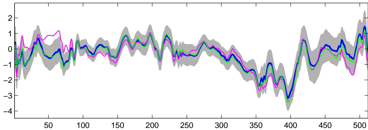
Estimated U_g(t) using G-WFMM: DE data, run 7
