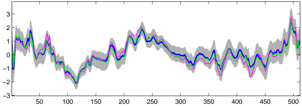
Estimated U_g(t) using G-WFMM: Normal data, run 7
