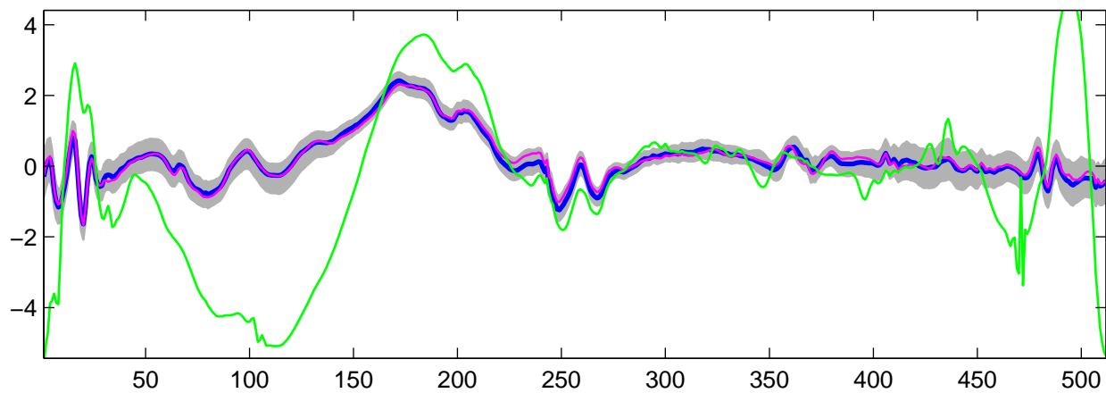
Estimated U_8(t) using R-WFMM: t_1 data, run 7
