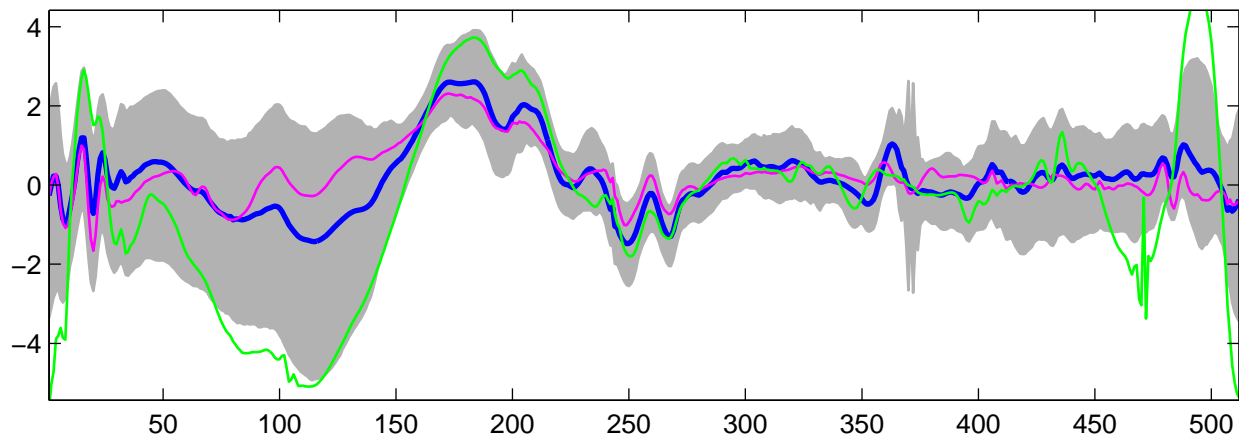
Estimated U_8(t) using G-WFMM: t_1 data, run 7
