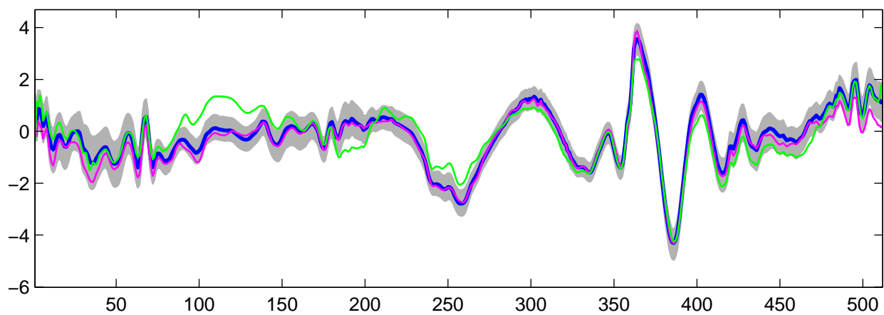
Estimated U_8(t) using R-WFMM: t_2 data, run 7
