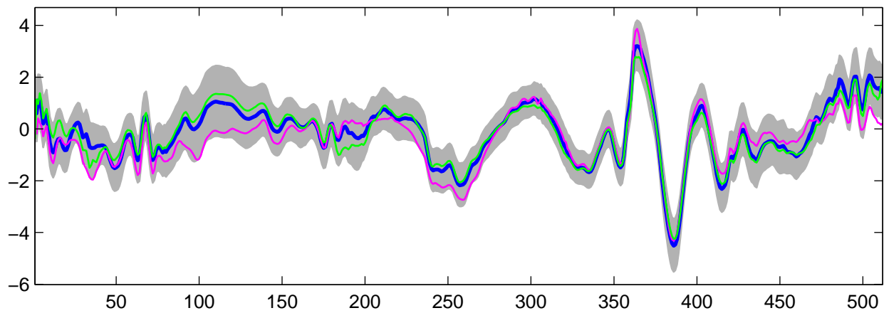
Estimated U_8(t) using G-WFMM: t_2 data, run 7
