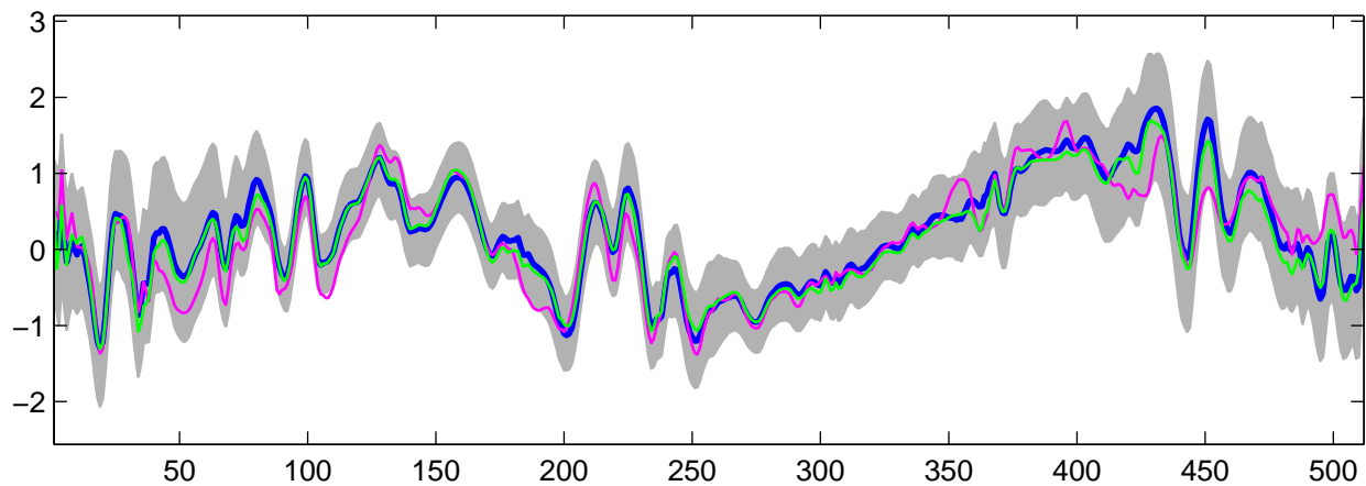
Estimated U_8(t) using G-WFMM: t_3 data, run 7
