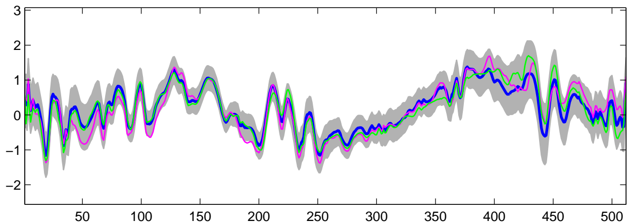
Estimated U_8(t) using R-WFMM: t_3 data, run 7
