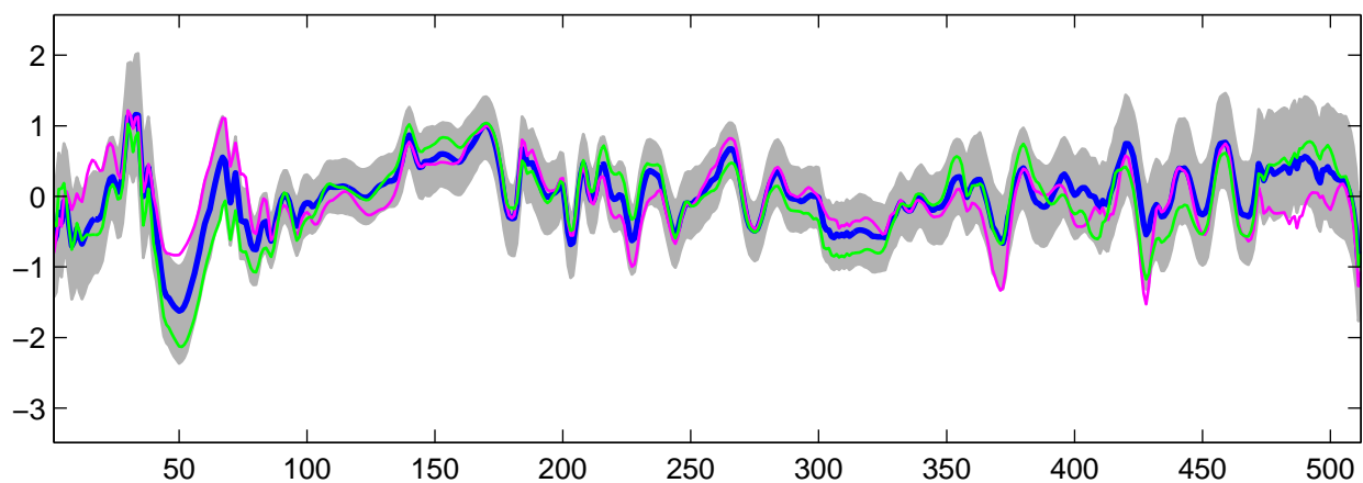
Estimated U_{\theta}(t) using R-WFMM: DE data, run 7
