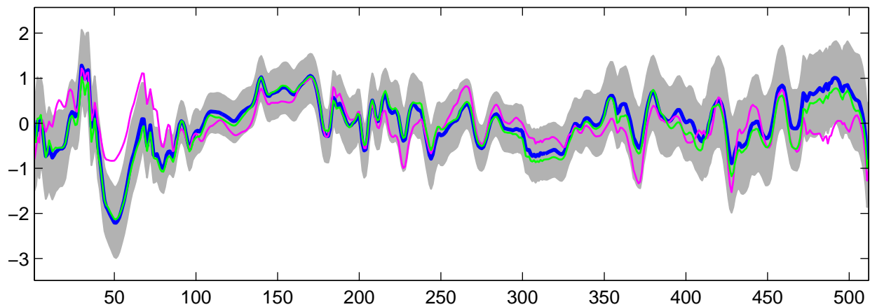
Estimated U_{\theta}(t) using G-WFMM: DE data, run 7
