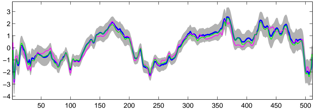
Estimated U_{\theta}(t) using G-WFMM: Normal data, run 7
