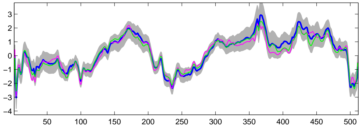
Estimated U_{\theta}(t) using R-WFMM: Normal data, run 7
