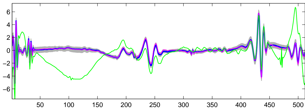
Estimated U_{\theta}(t) using R-WFMM: t_1 data, run 7
