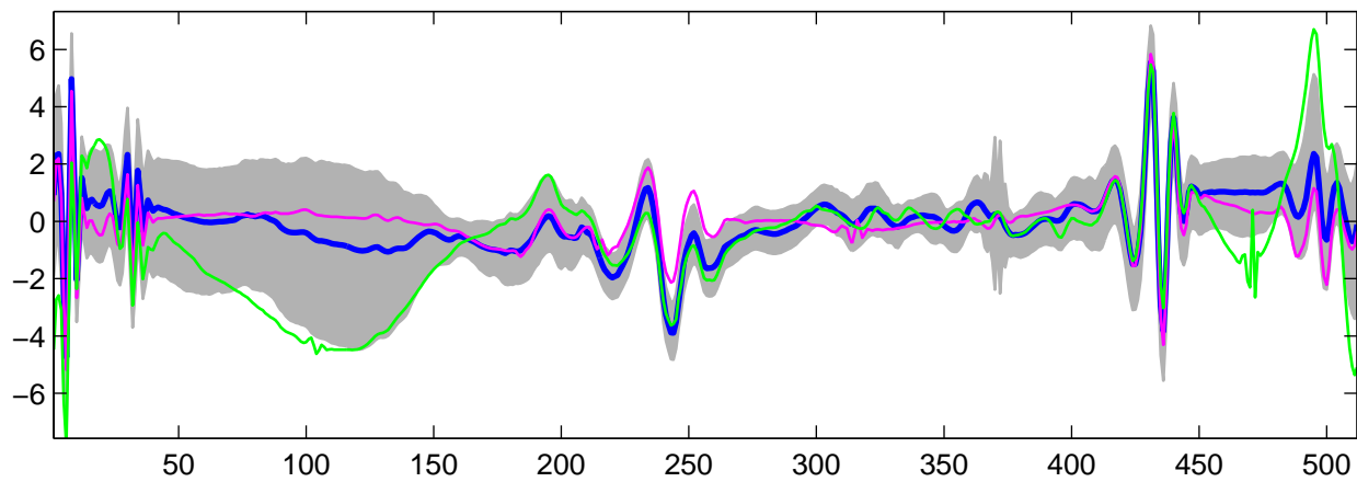
Estimated U_{\theta}(t) using G-WFMM: t_1 data, run 7
