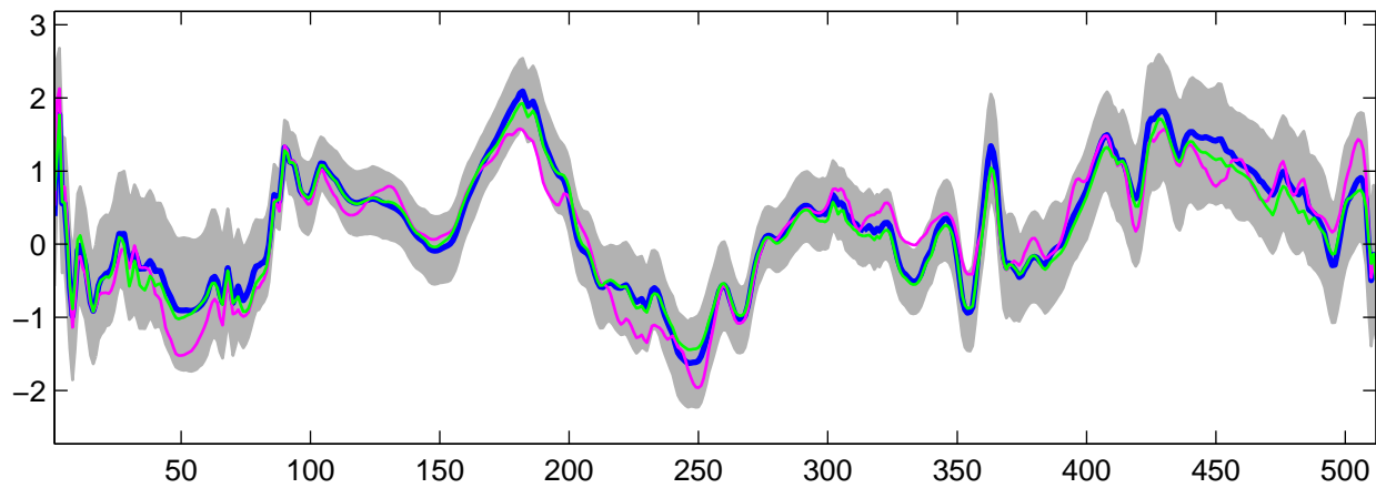
Estimated U_9(t) using G-WFMM: t_3 data, run 7
