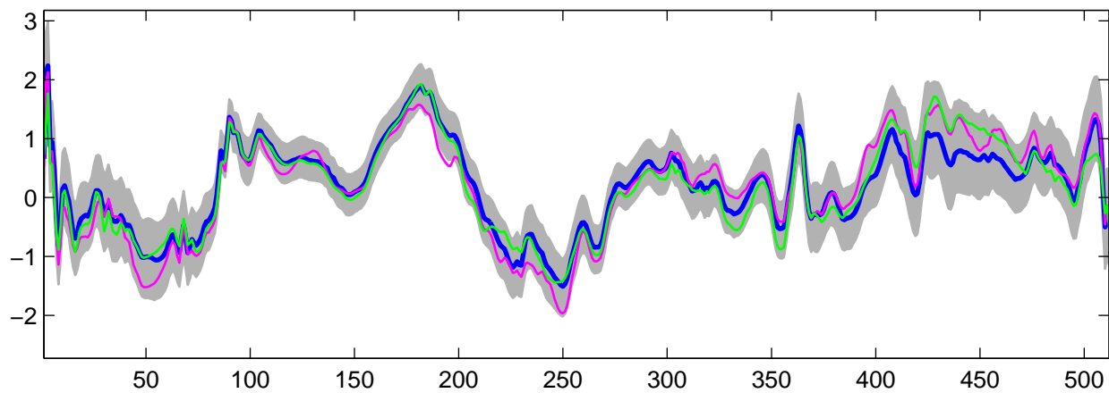
Estimated U_9(t) using R-WFMM: t_3 data, run 7
