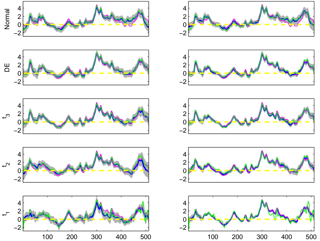
The estimated B_1(t) for 5 simulated datasets, simulation run 8 G-WFMM R-WFMM
