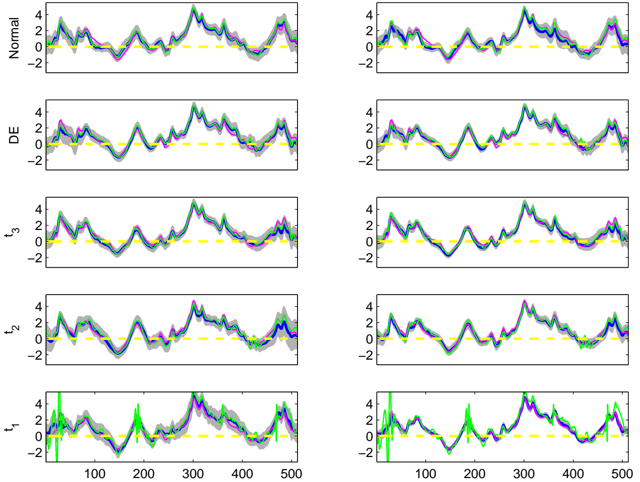
The estimated B_2(t) for 5 simulated datasets, simulation run 8 G-WFMM R-WFMM
