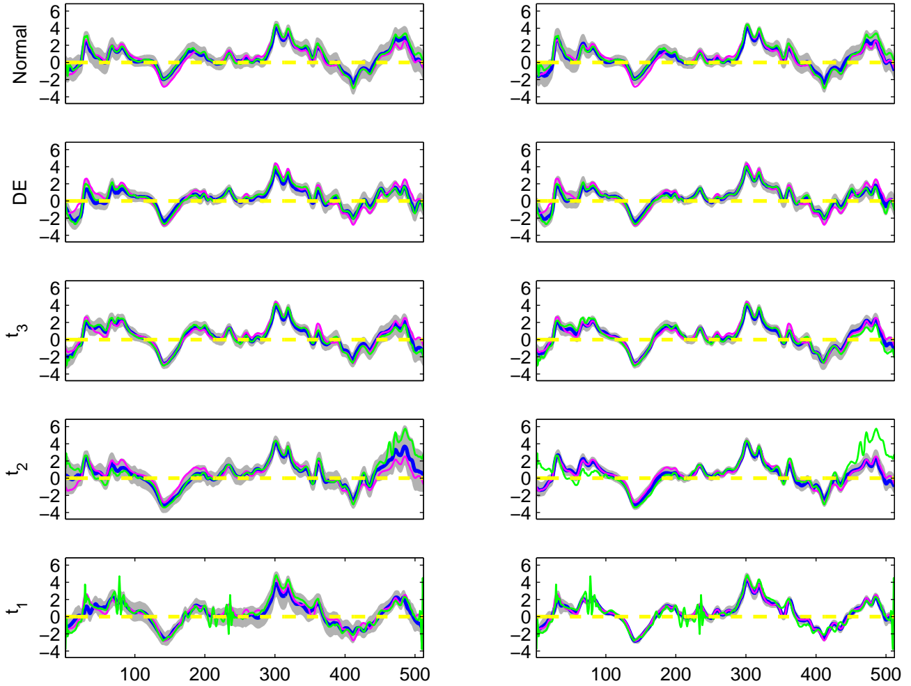
The estimated B_3(t) for 5 simulated datasets, simulation run 8 G-WFMM R-WFMM
