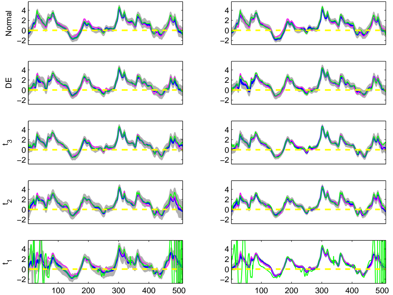
The estimated B_4(t) for 5 simulated datasets, simulation run 8 G-WFMM R-WFMM
