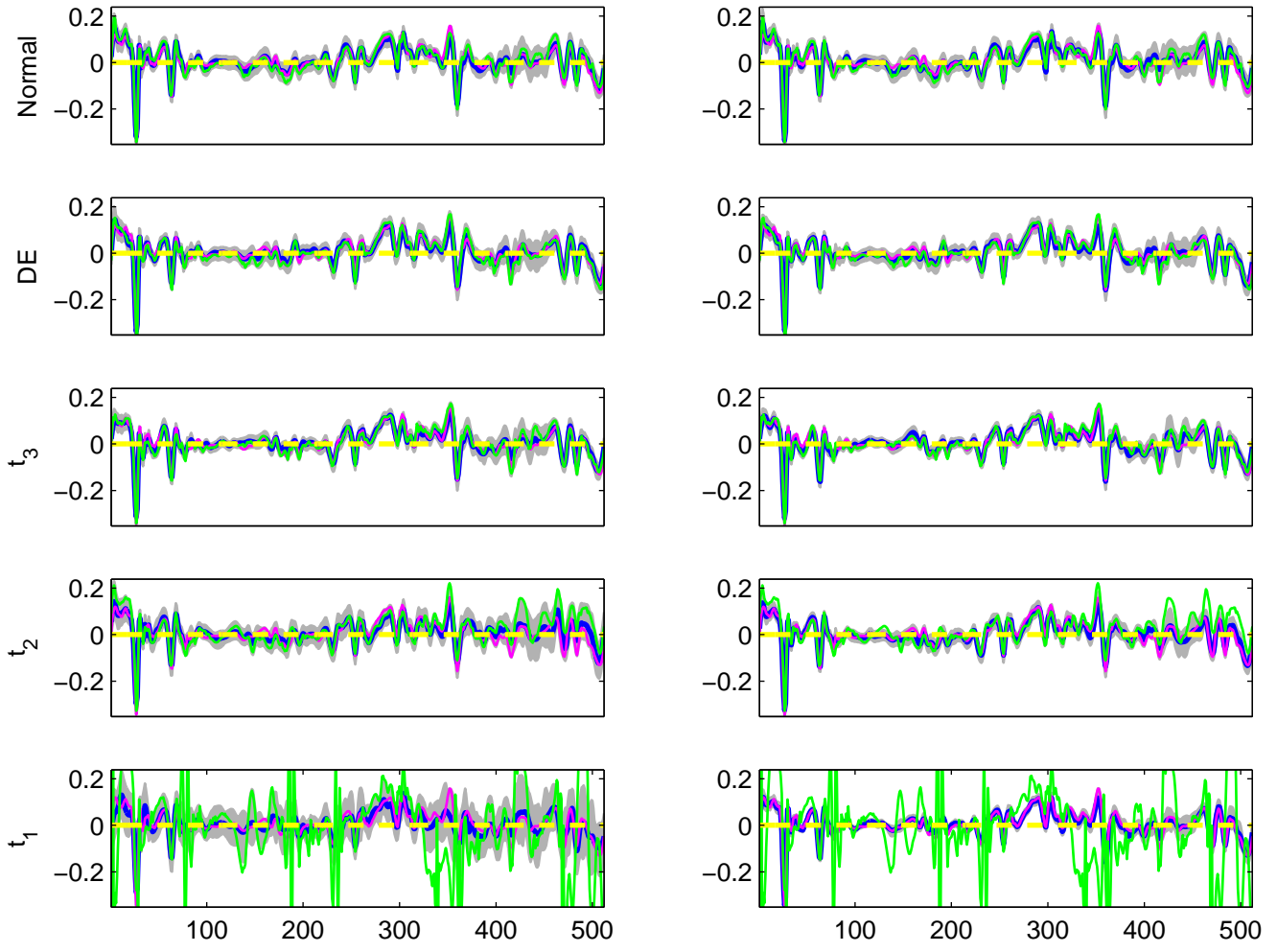
The estimated B_5(t) for 5 simulated datasets, simulation run 8 G-WFMM R-WFMM
