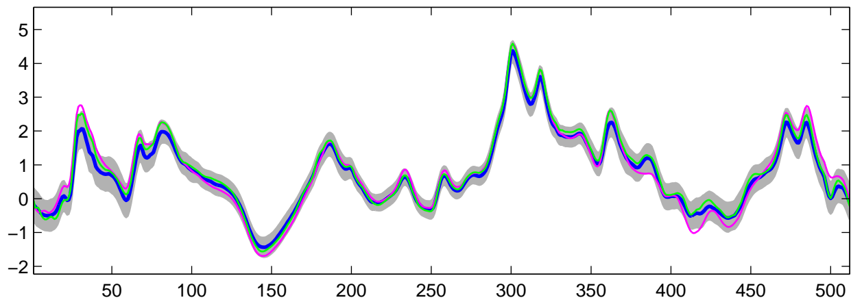
Estimated C_0(t) using G-WFMM: DE data, run 8
