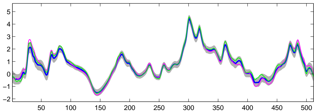
Estimated C_0(t) using R-WFMM: DE data, run 8
