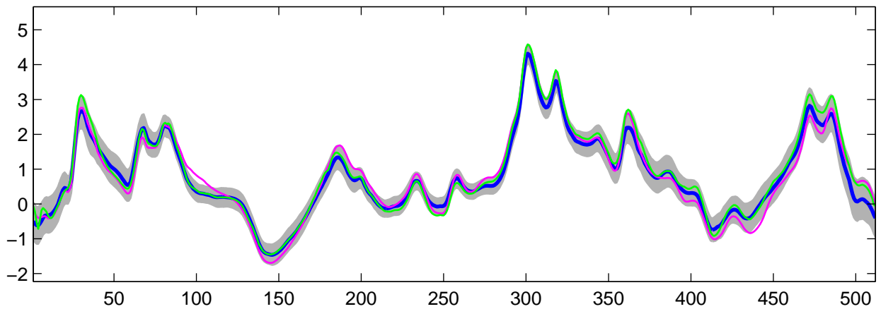
Estimated C_0(t) using R-WFMM: Normal data, run 8
