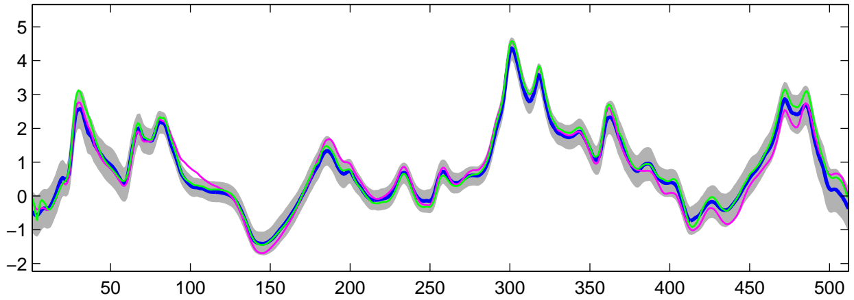
Estimated C_0(t) using G-WFMM: Normal data, run 8
