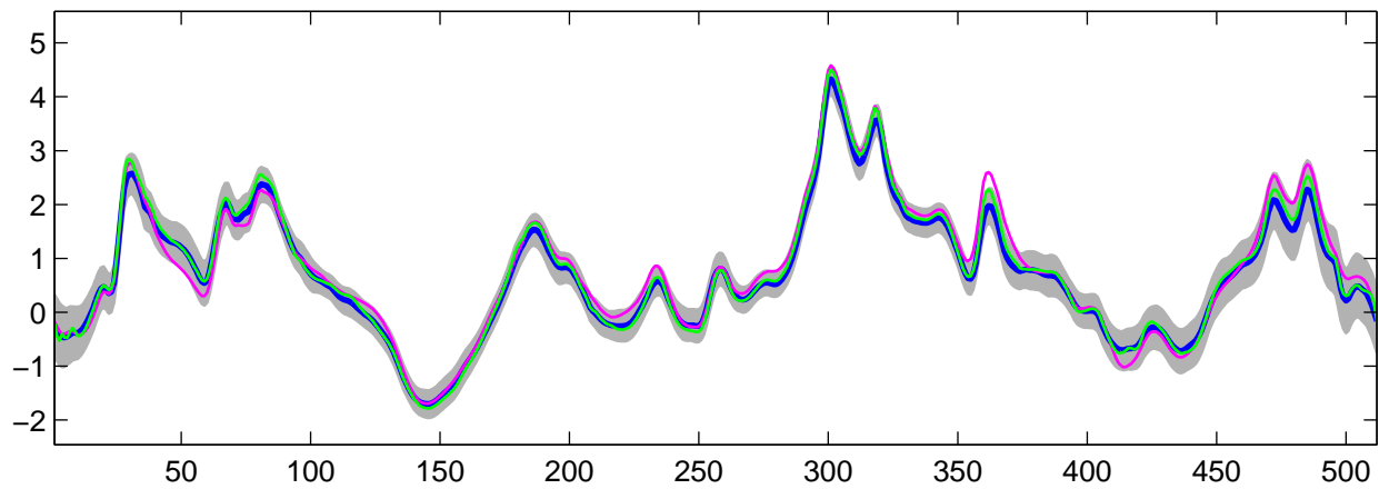
Estimated C_0(t) using G-WFMM: t_3 data, run 8
