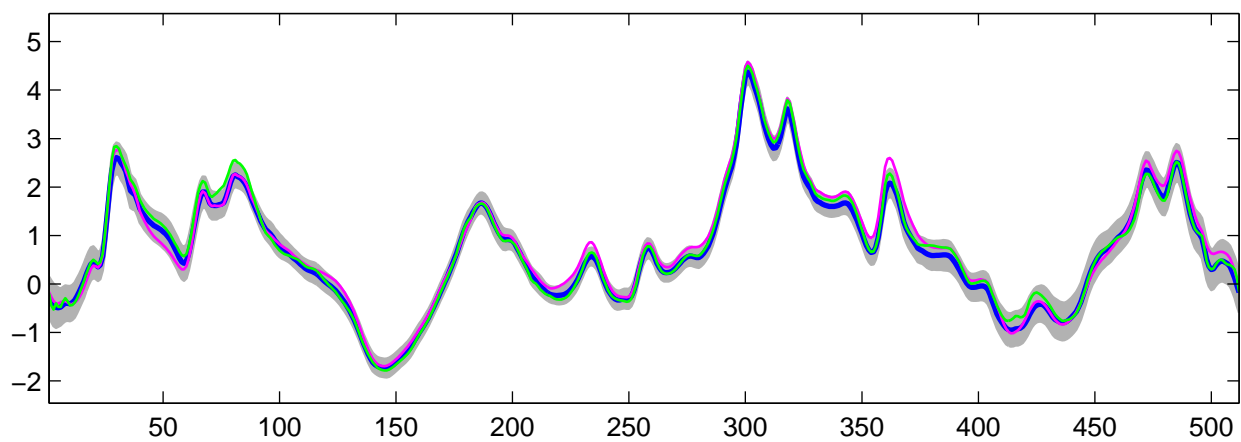
Estimated C_0(t) using R-WFMM: t_3 data, run 8
