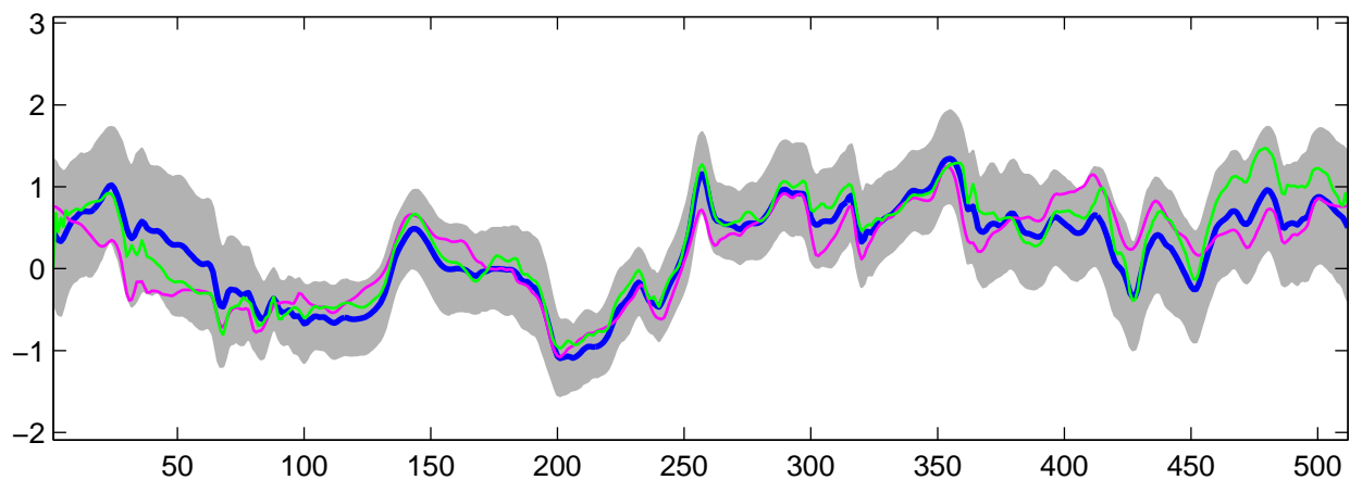
Estimated C_1(t) using R-WFMM: DE data, run 8
