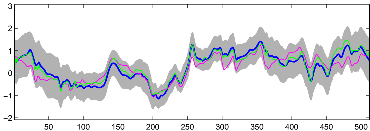
Estimated C_1(t) using G-WFMM: DE data, run 8
