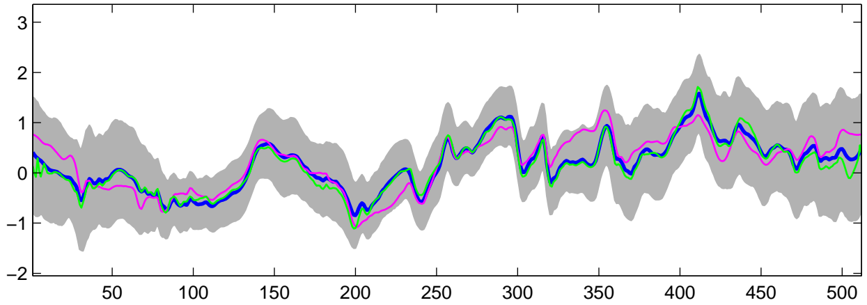
Estimated C_1(t) using G-WFMM: Normal data, run 8
