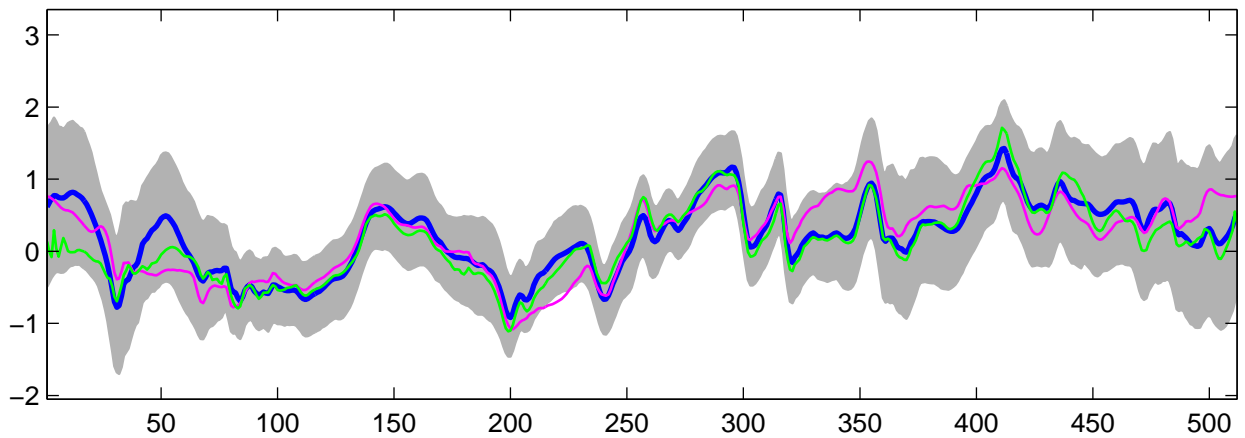
Estimated C_1(t) using R-WFMM: Normal data, run 8
