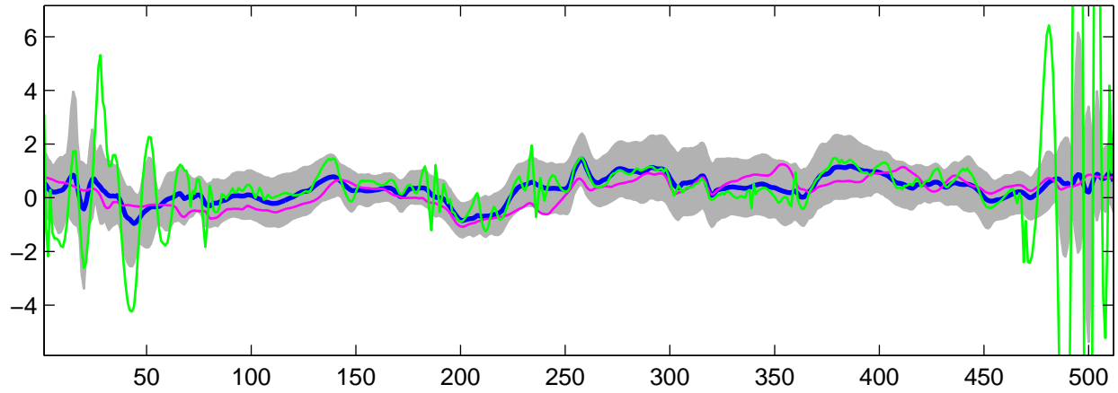
Estimated C_1(t) using G-WFMM: t_1 data, run 8
