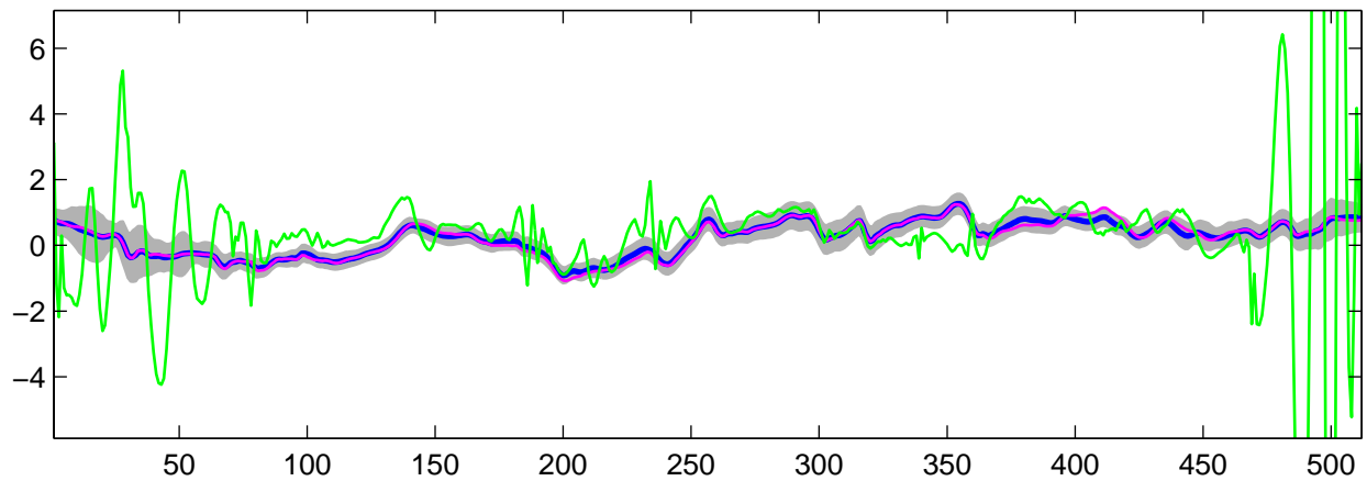
Estimated C_1(t) using R-WFMM: t_1 data, run 8
