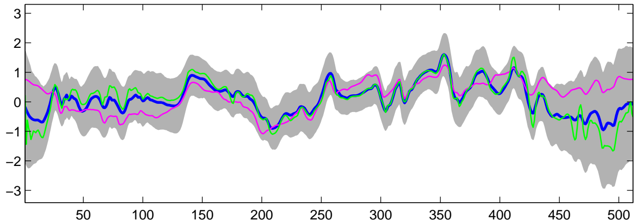
Estimated C_1(t) using G-WFMM: t_2 data, run 8
