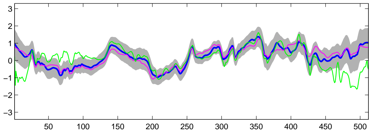
Estimated C_1(t) using R-WFMM: t_2 data, run 8
