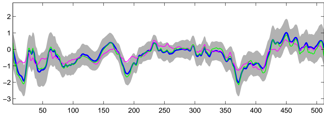
Estimated C_2(t) using G-WFMM: DE data, run 8
