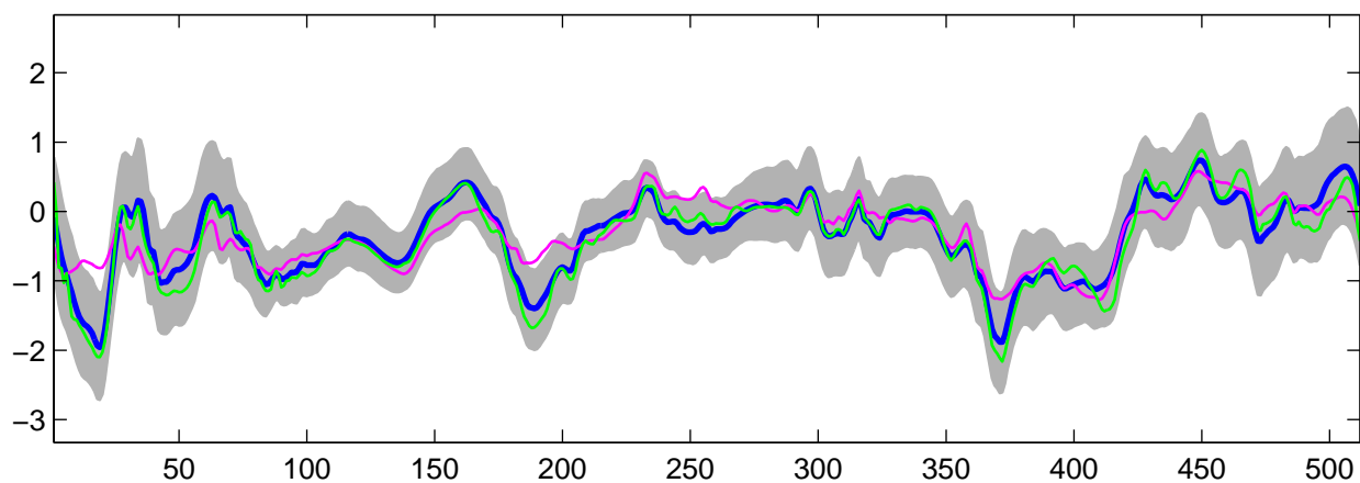
Estimated C_2(t) using R-WFMM: DE data, run 8
