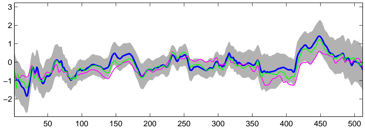
Estimated C_2(t) using R-WFMM: Normal data, run 8
