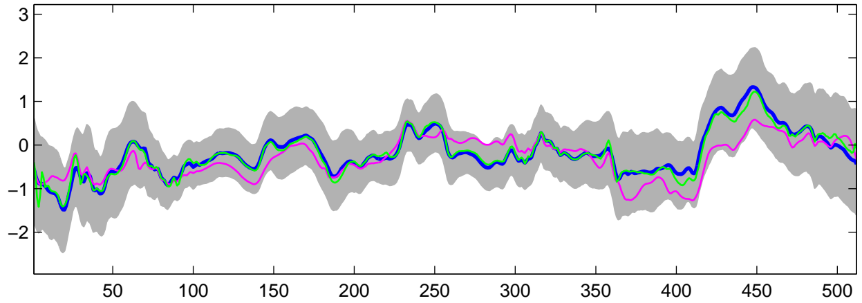
Estimated C_2(t) using G-WFMM: Normal data, run 8
