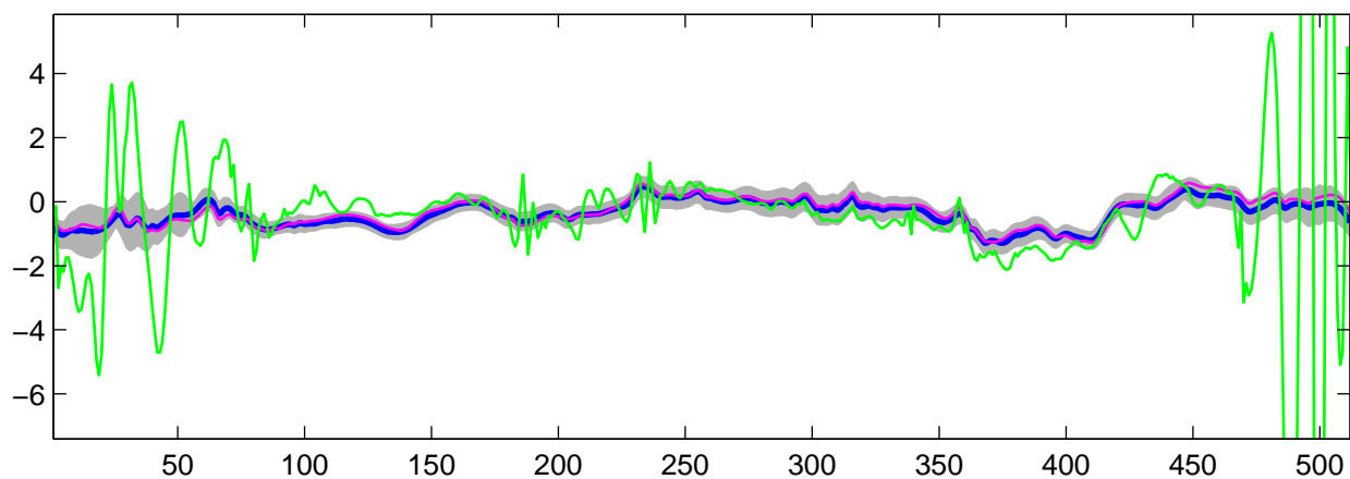
Estimated C_2(t) using R-WFMM: t_1 data, run 8
