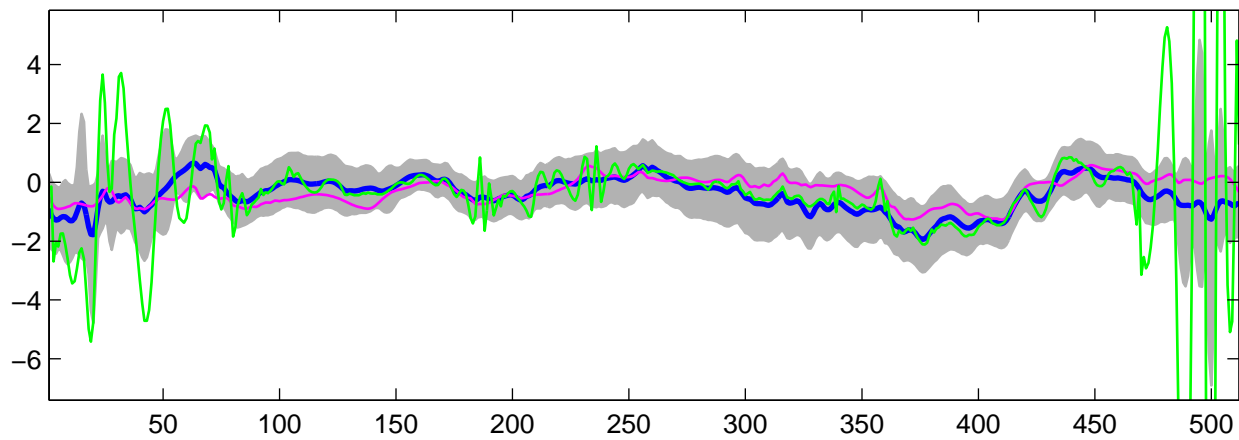
Estimated C_2(t) using G-WFMM: t_1 data, run 8
