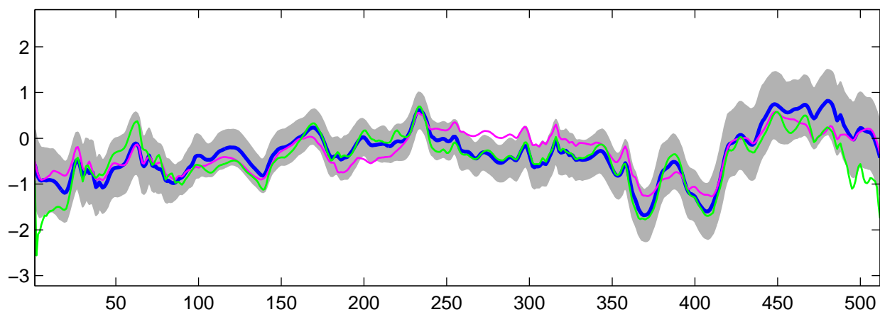
Estimated C_2(t) using R-WFMM: t_3 data, run 8
