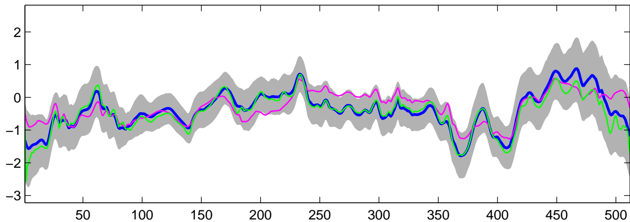
Estimated C_2(t) using G-WFMM: t_3 data, run 8
