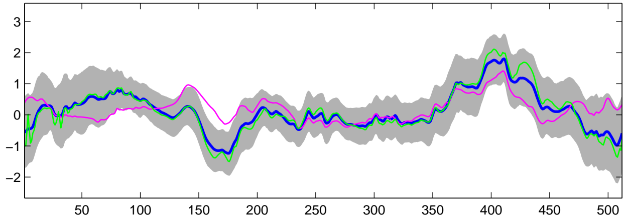
Estimated C_3(t) using G-WFMM: Normal data, run 8
