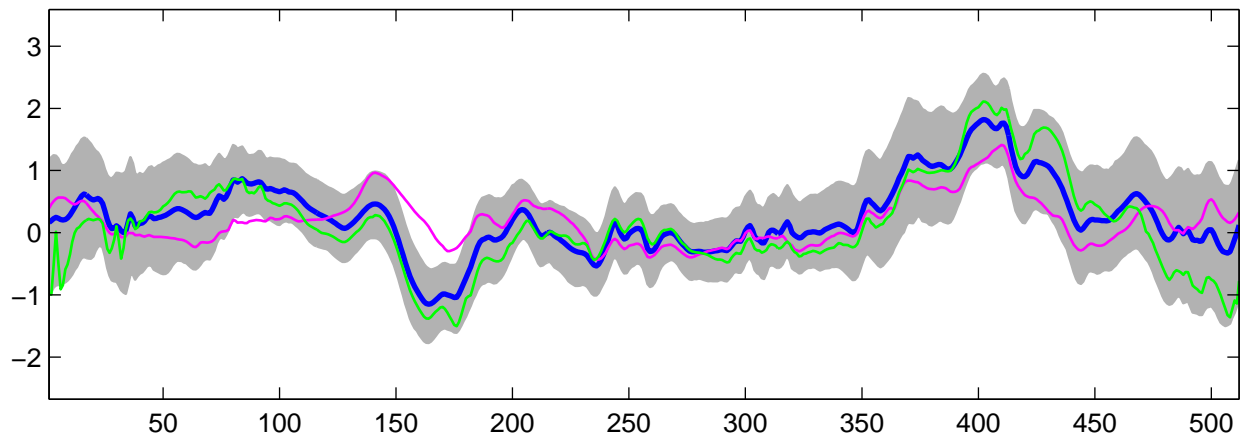
Estimated C_3(t) using R-WFMM: Normal data, run 8
