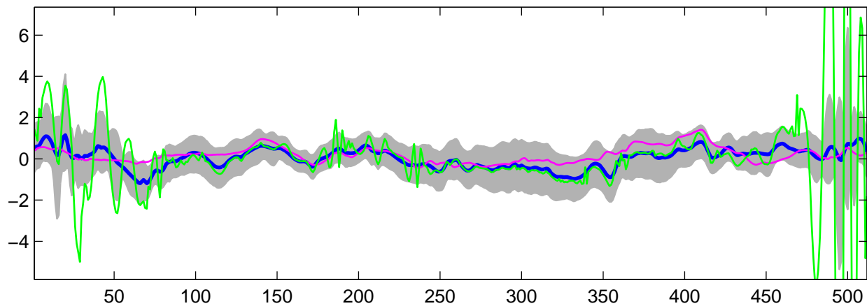
Estimated C_3(t) using G-WFMM: t_1 data, run 8
