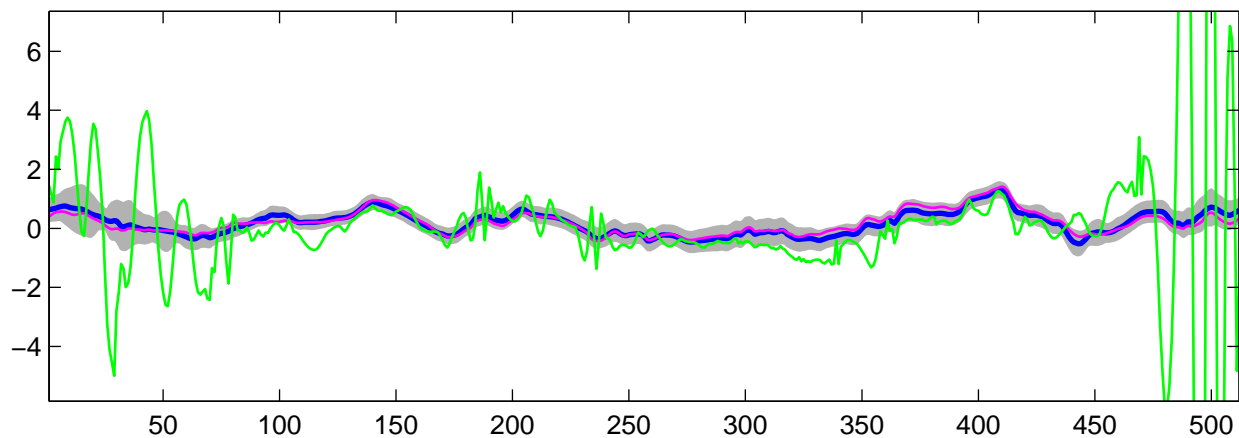
Estimated C_3(t) using R-WFMM: t_1 data, run 8
