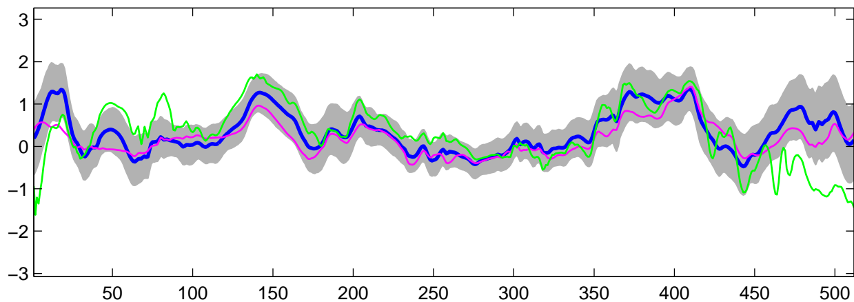
Estimated C_3(t) using R-WFMM: t_2 data, run 8
