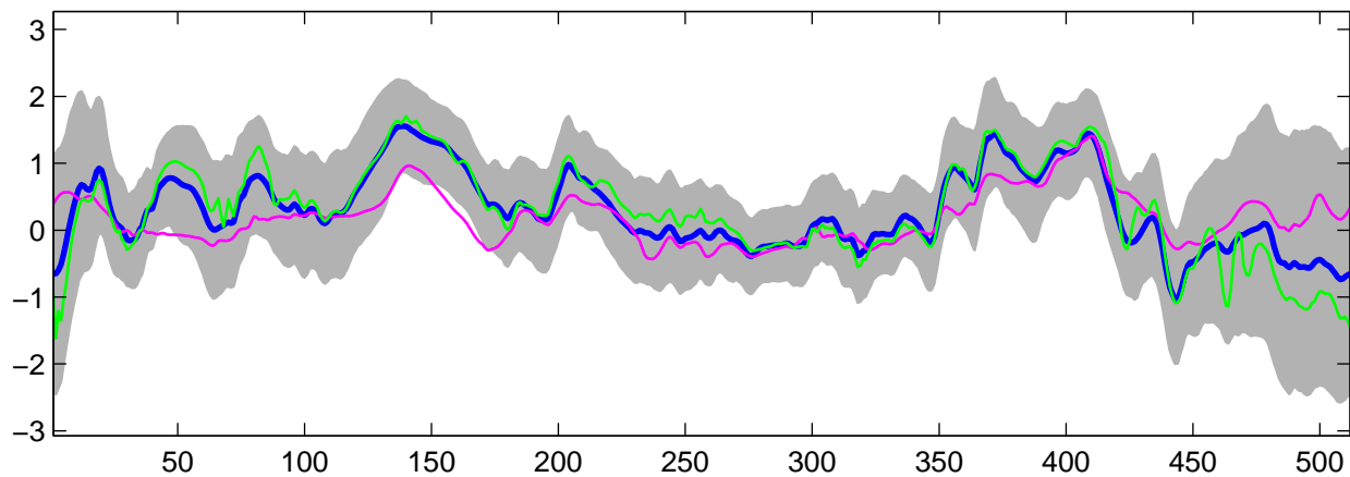
Estimated C_3(t) using G-WFMM: t_2 data, run 8
