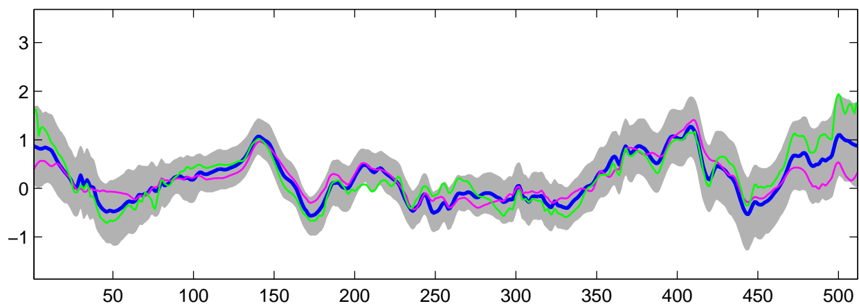
Estimated C_3(t) using R-WFMM: t_3 data, run 8
