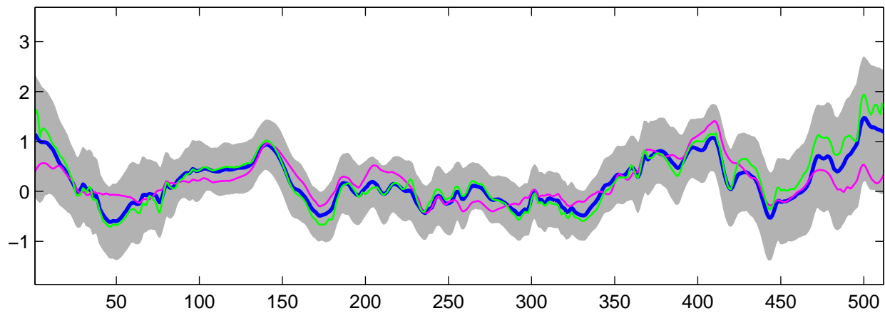
Estimated C_3(t) using G-WFMM: t_3 data, run 8
