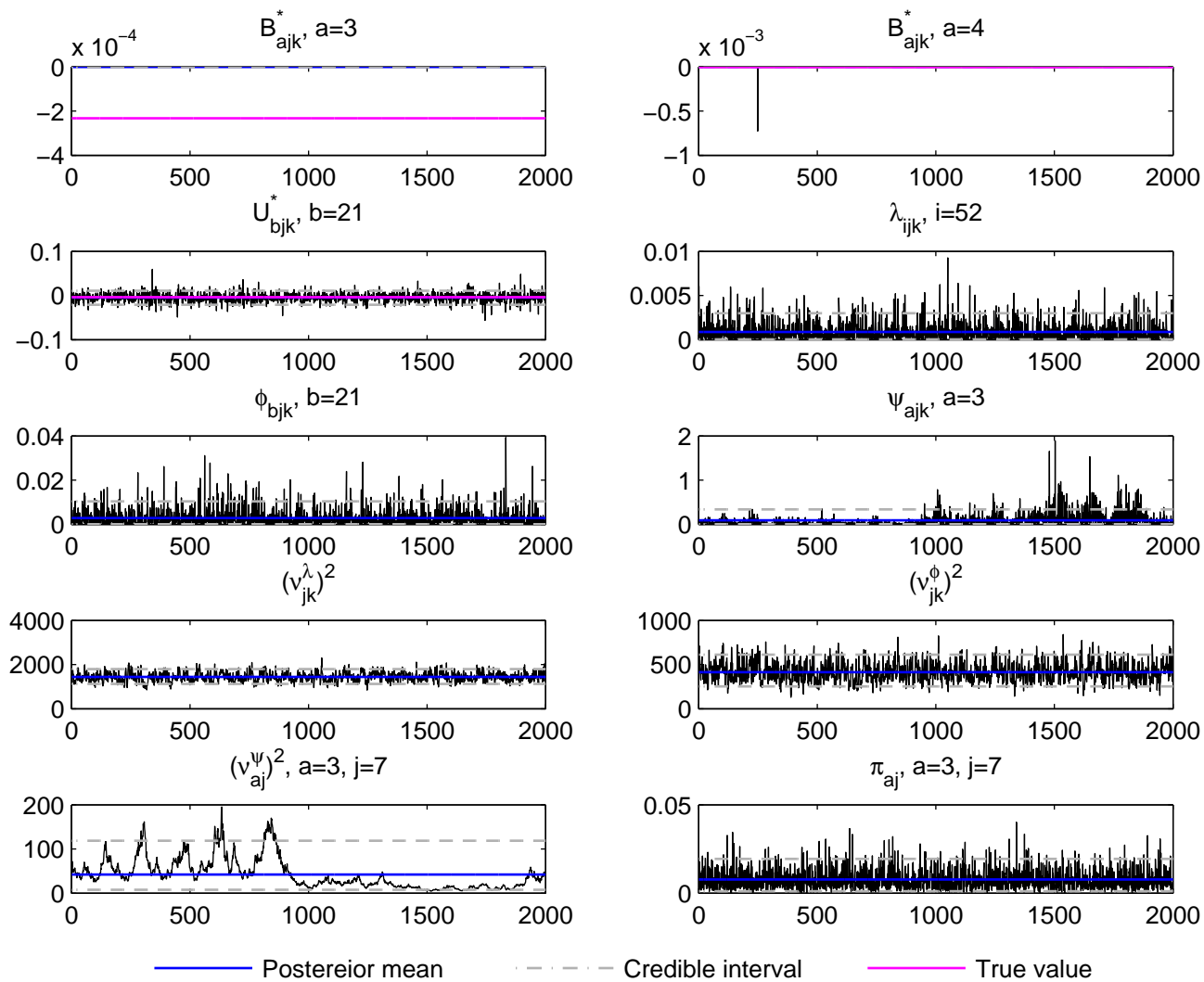
Trace plot, j=7, k=2 , DE data, simulation run 8
