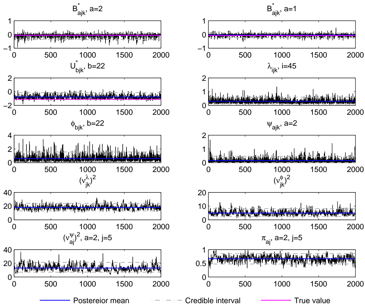
Trace plot, j=5, k=1 , Normal data, simulation run 8
