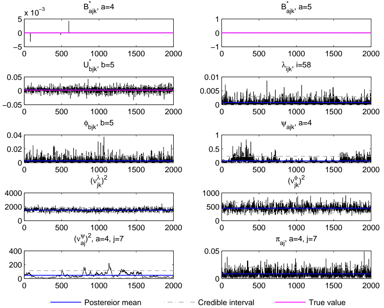
Trace plot, j=7, k=2, t_j data, simulation run 8
