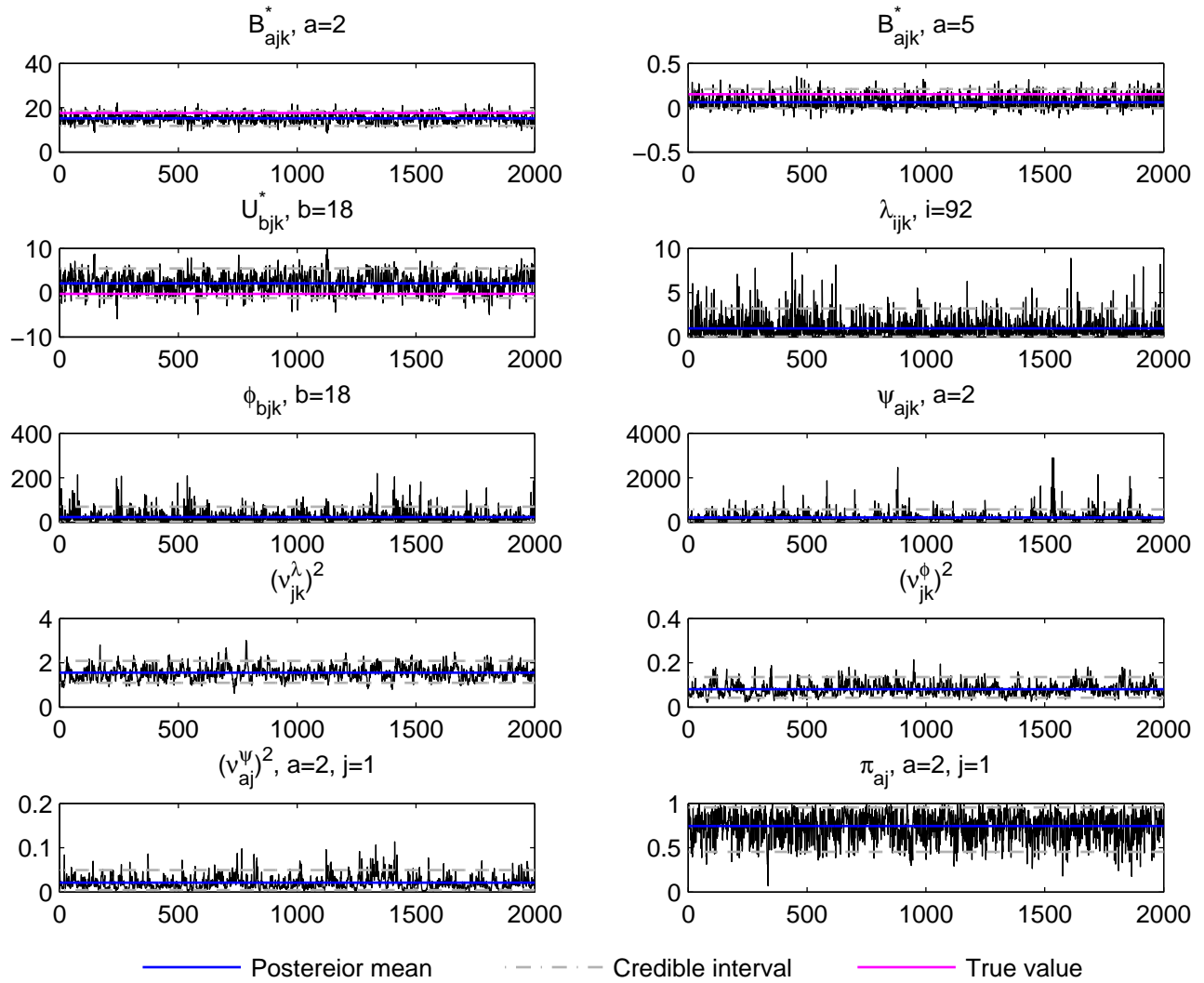
Trace plot, j=1, k=2, t_3 data, simulation run 8
