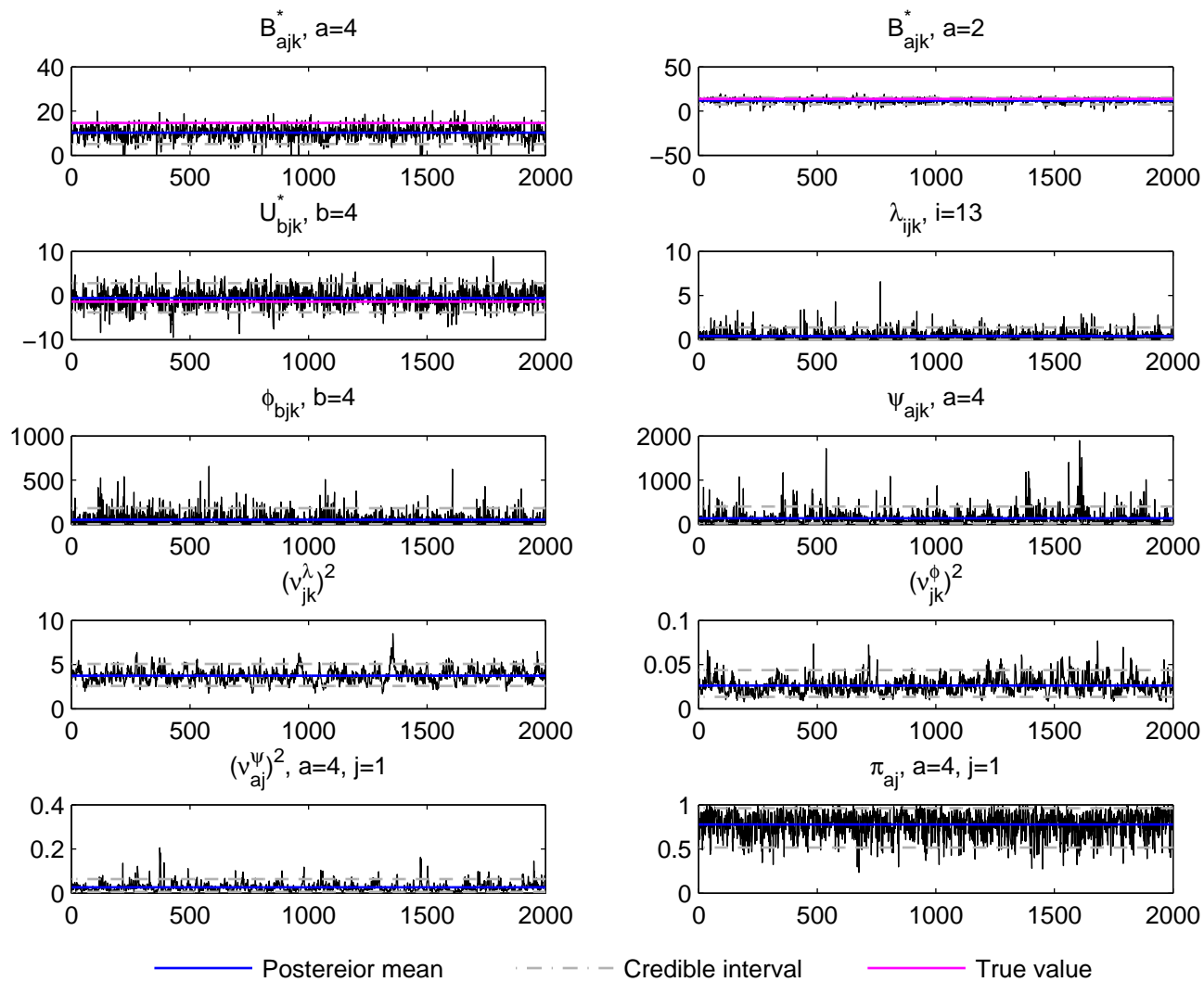
Trace plot, j=1, k=5 , DE data, simulation run 8
