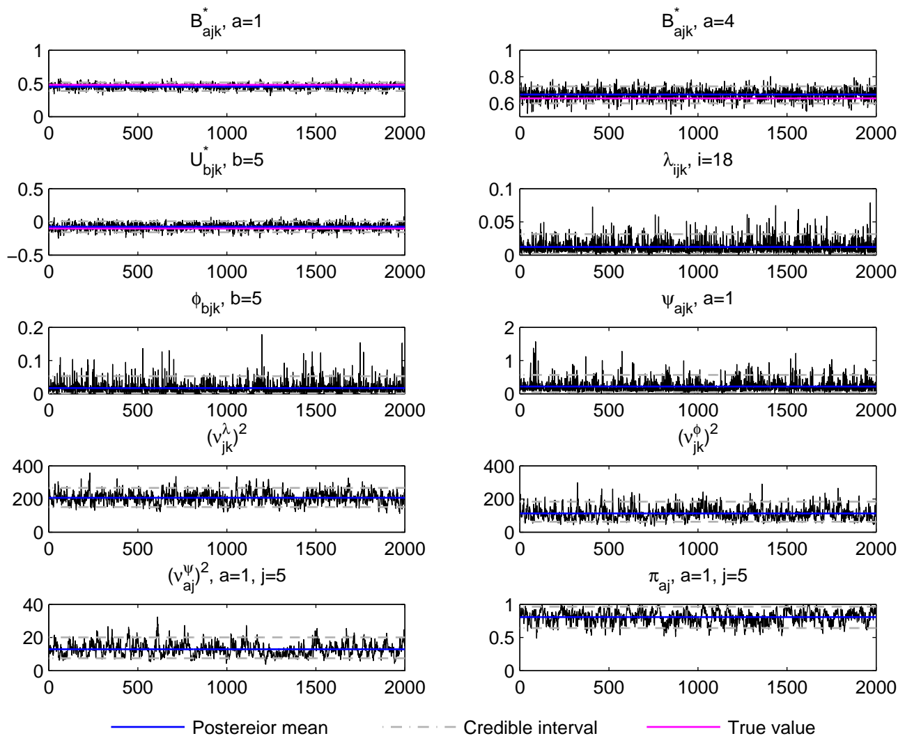
Trace plot, j=5, k=5 , Normal data, simulation run 8
