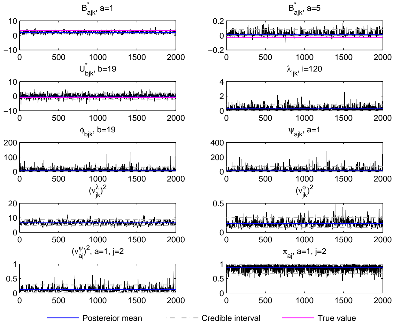
Trace plot, j=2, k=1, t_2 data, simulation run 8
