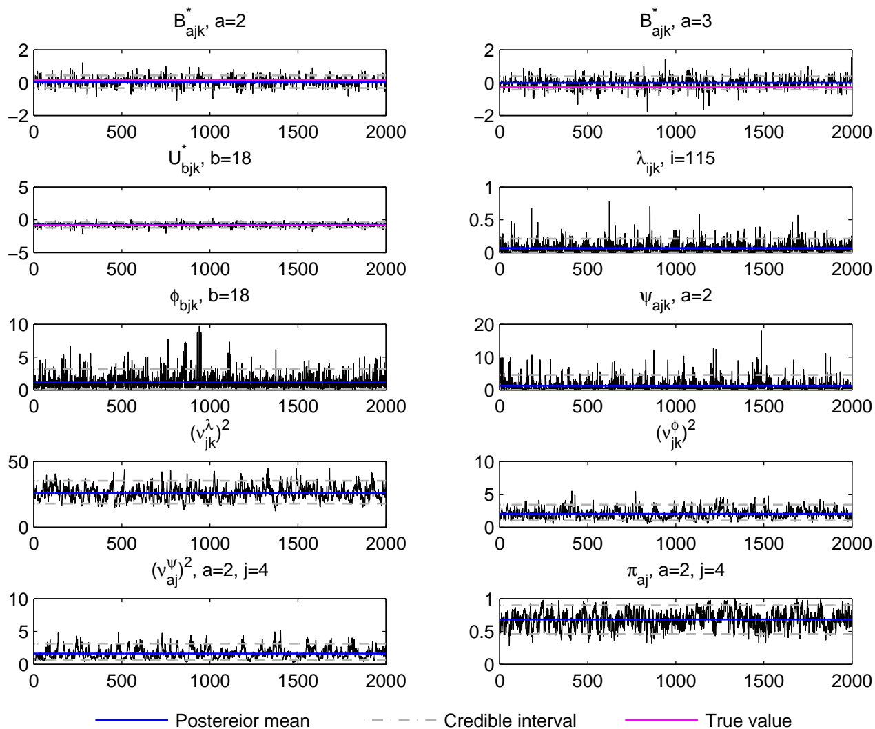
Trace plot, j=4, k=2 , DE data, simulation run 8
