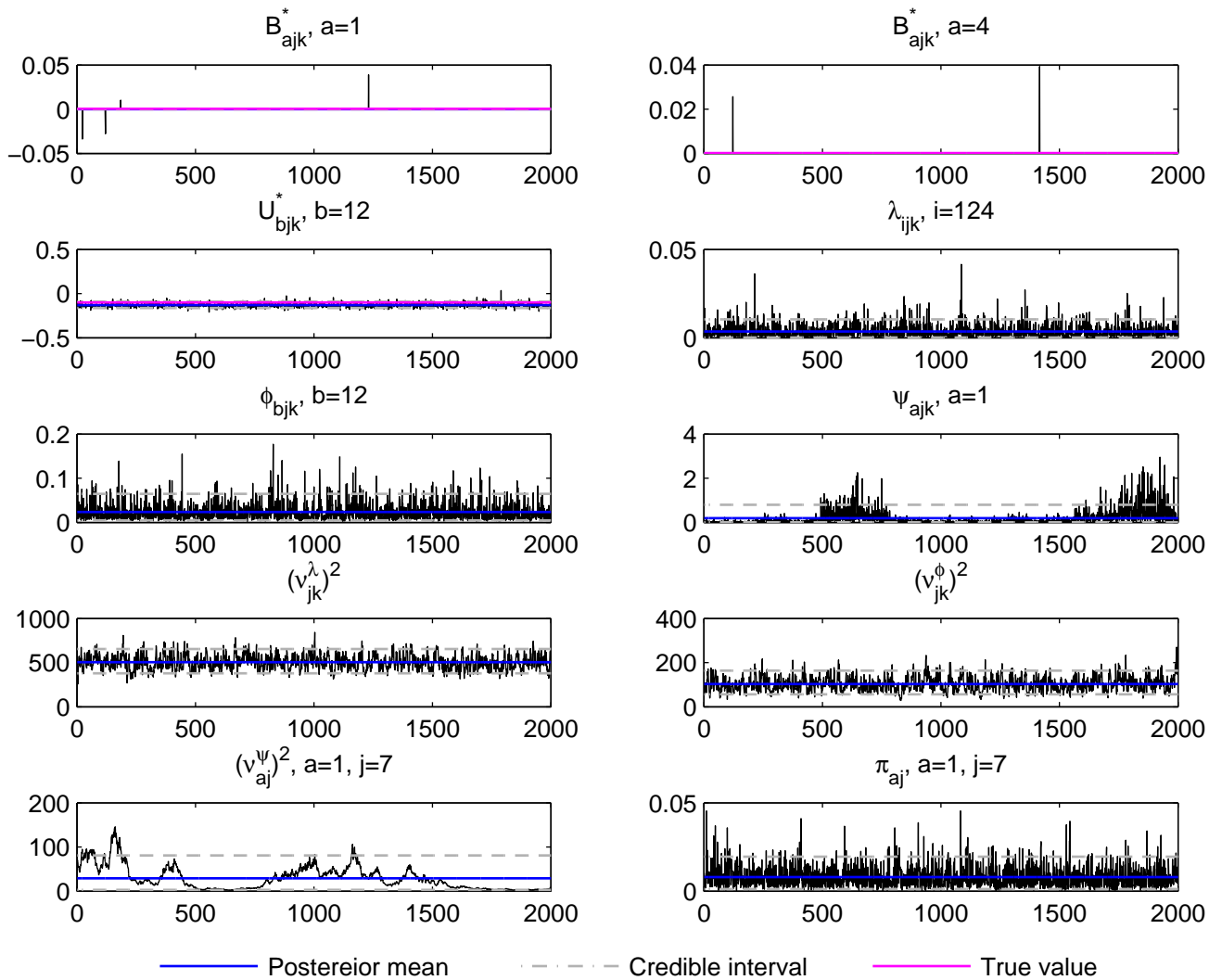
Trace plot, j=7, k=1 , Normal data, simulation run 8
