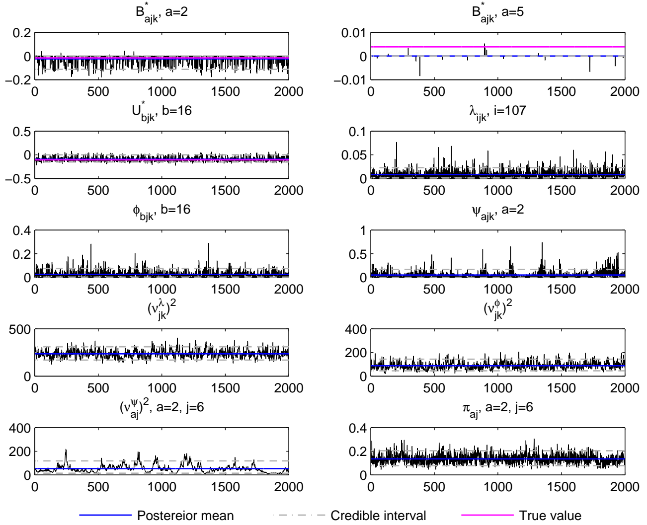
Trace plot, j=6, k=1, t_j data, simulation run 8
