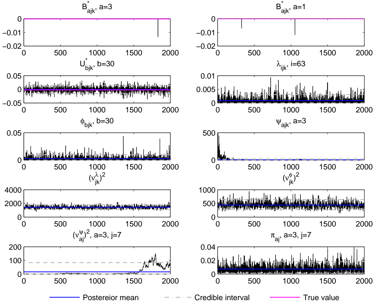
Trace plot, j=7, k=2, t_2 data, simulation run 8
