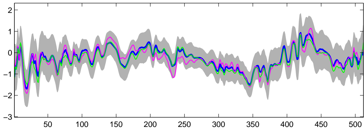
Estimated U_{10}(t) using G-WFMM: DE data, run 8
