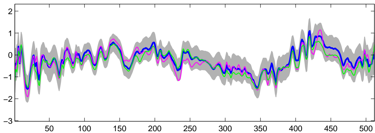
Estimated U_{10}(t) using R-WFMM: DE data, run 8
