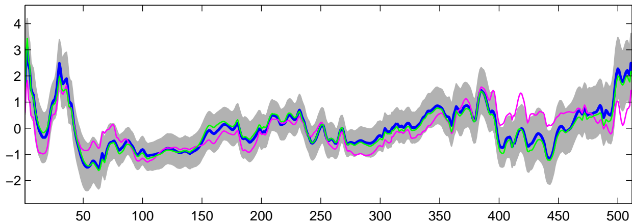
Estimated U_{10}(t) using G-WFMM: Normal data, run 8
