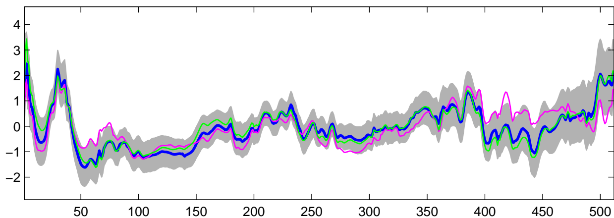
Estimated U_{10}(t) using R-WFMM: Normal data, run 8
