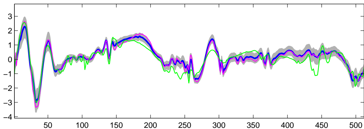
Estimated U_{10}(t) using R-WFMM: t_1 data, run 8
