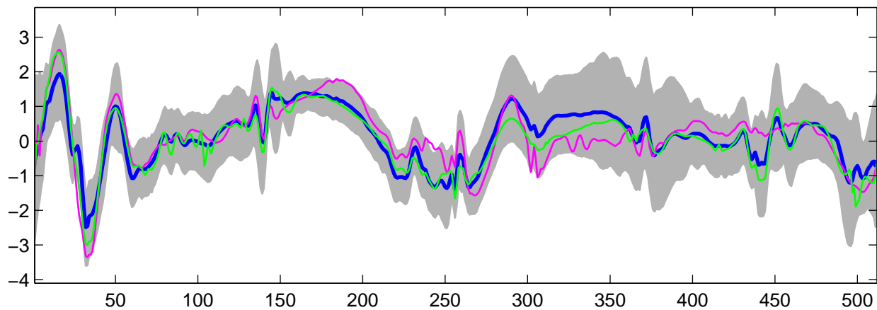
Estimated U_{10}(t) using G-WFMM: t_1 data, run 8
