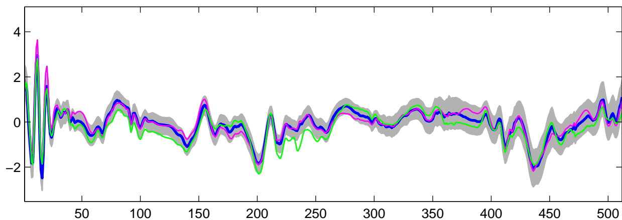
Estimated U_{10}(t) using R-WFMM: t_2 data, run 8
