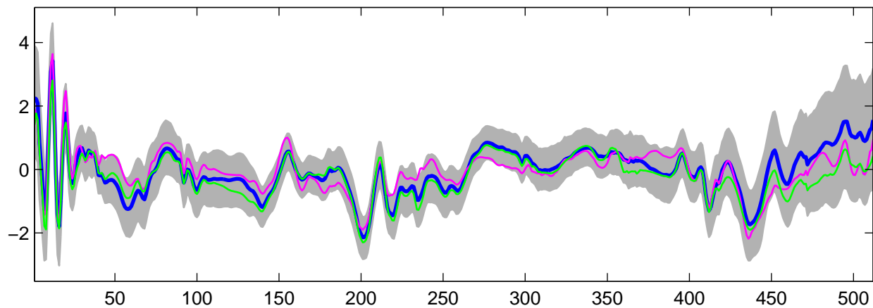
Estimated U_{10}(t) using G-WFMM: t_2 data, run 8
