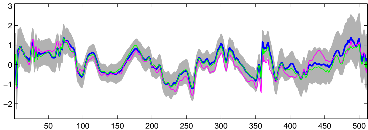
Estimated U_{10}(t) using G-WFMM: t_3 data, run 8
