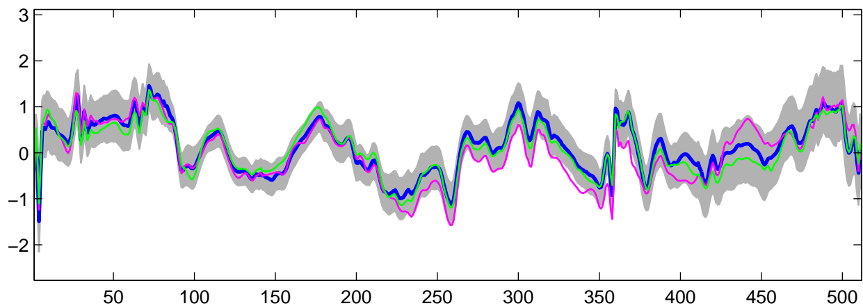
Estimated U_{10}(t) using R-WFMM: t_3 data, run 8
