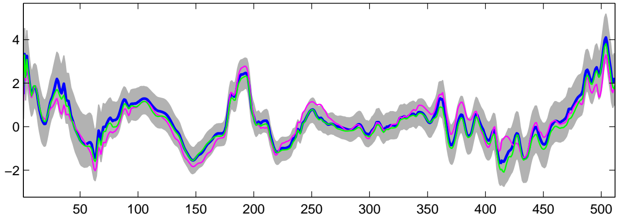
Estimated U_{11}(t) using G-WFMM: DE data, run 8
