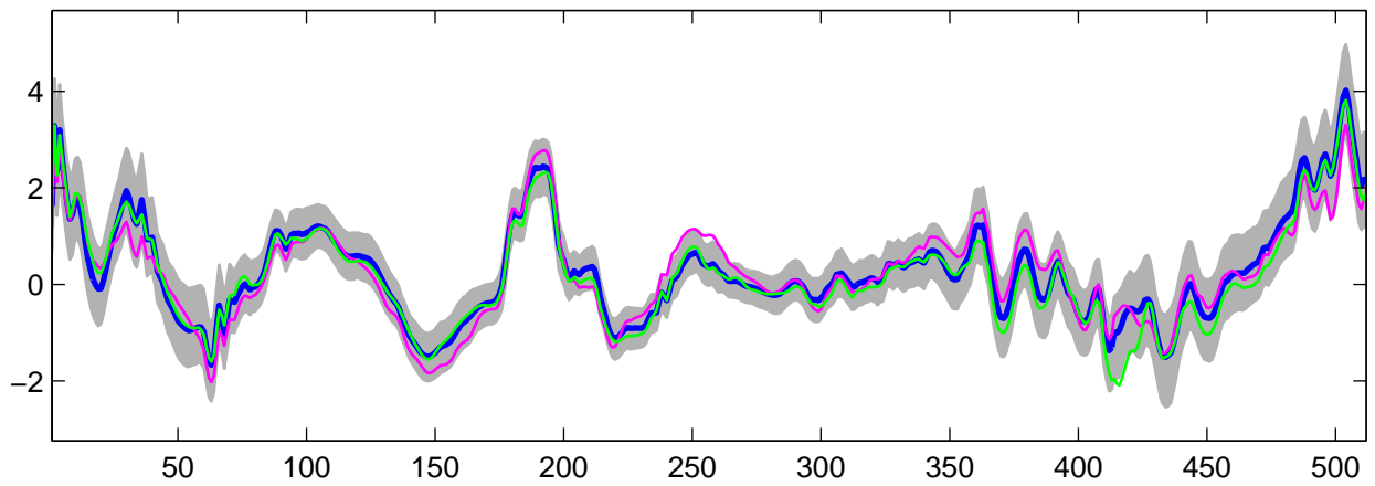
Estimated U_{11}(t) using R-WFMM: DE data, run 8
